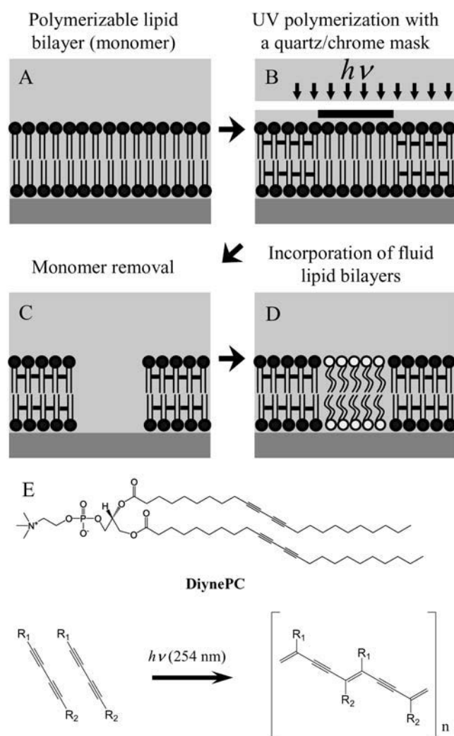
FIGURE 1 (A–D) Schematic outline of the bilayer patterning procedure. (E) The chemical structure of polymerizable diacylene phospholipid, DiynePC, and its photopolymerization scheme.
